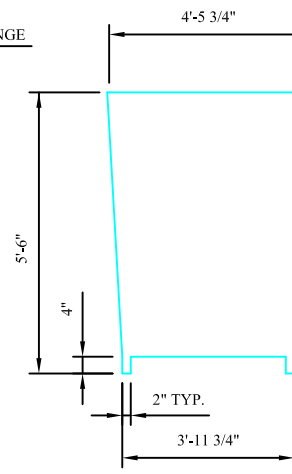
BAFFLE WALL DETAIL
