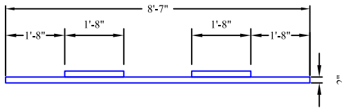
COVER ELEVATION VIEW
