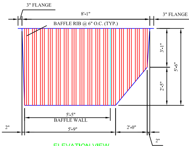
ELEVATION VIEW
