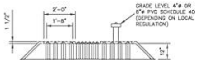
COVER ELEVATION VIEW
