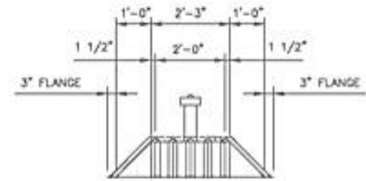
COVER ELEVATION VIEW
