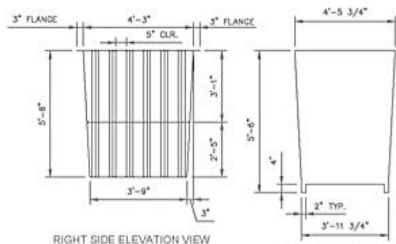
BAFFLE WALL DETAIL
