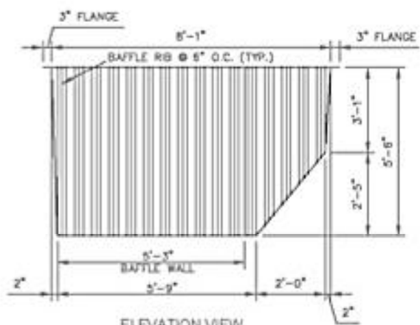
ELEVATION VIEW
